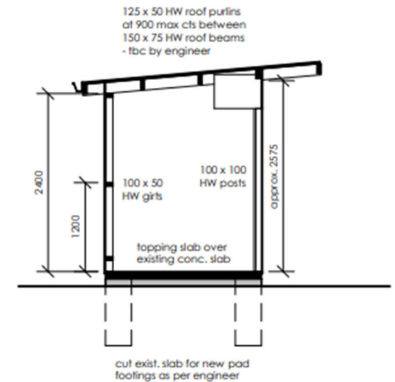
section thru
