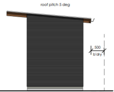
east elevation
