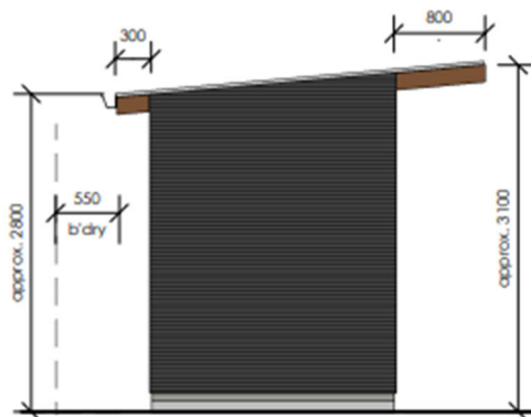
west elevation
