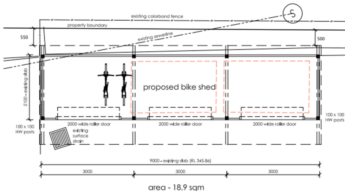
bike storage shed - floor plan
